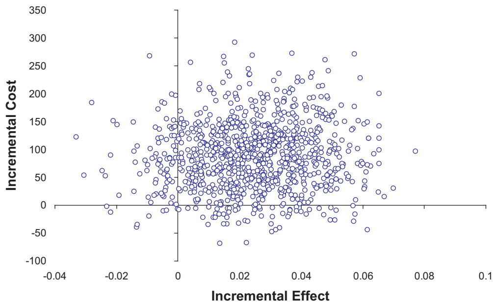
FIGURE 1 Cost-utility plane
